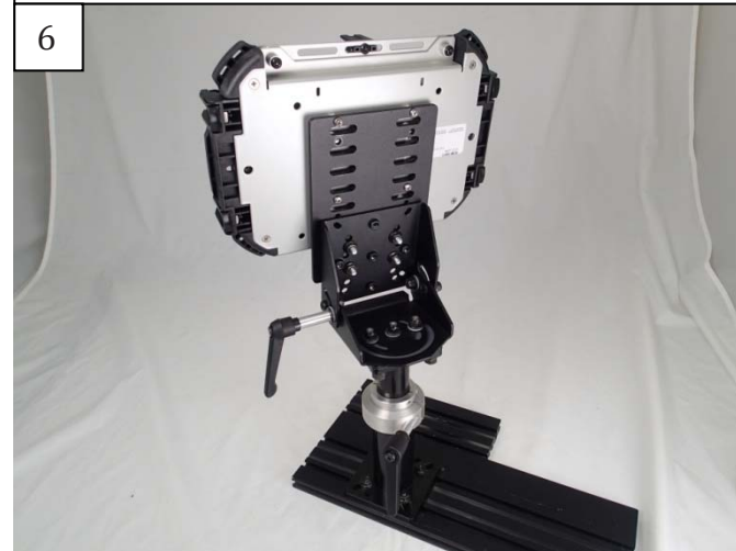
UT-201 on C-MM-218 with C-MD-202 shown on C-HDM-301 on C-HDM-201
