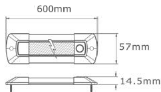
Infrared sensor
